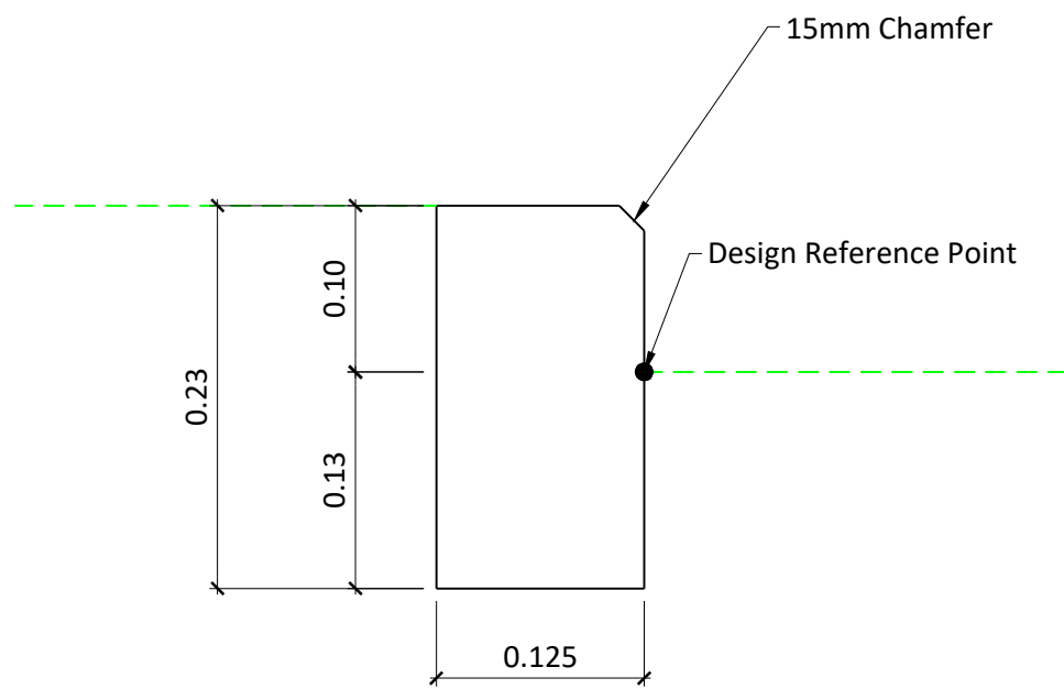
STANDARD NIB Scale 1:5
