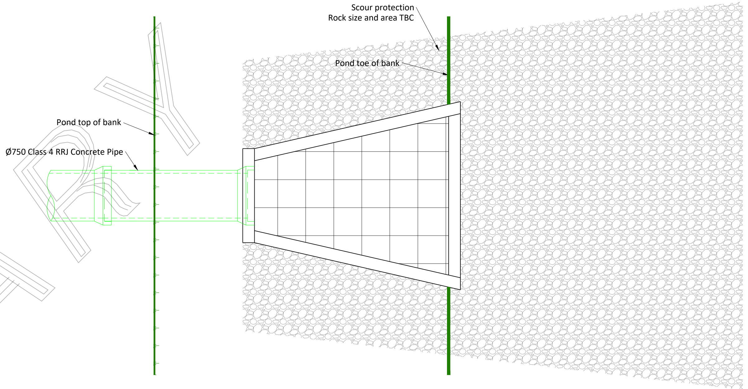
INLET STRUCTURE PLAN VIEW Scale 1:40
