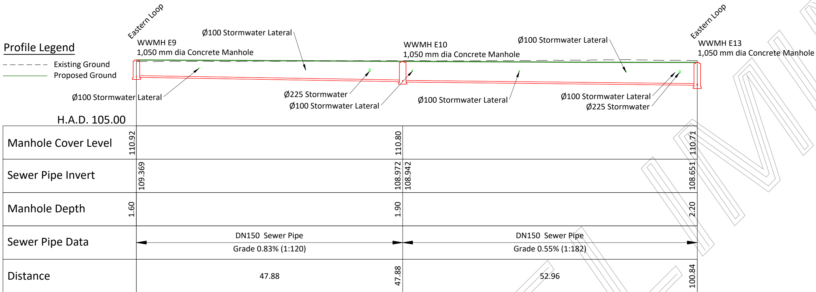
Longsection: WWMH E9 to WWMH 13
