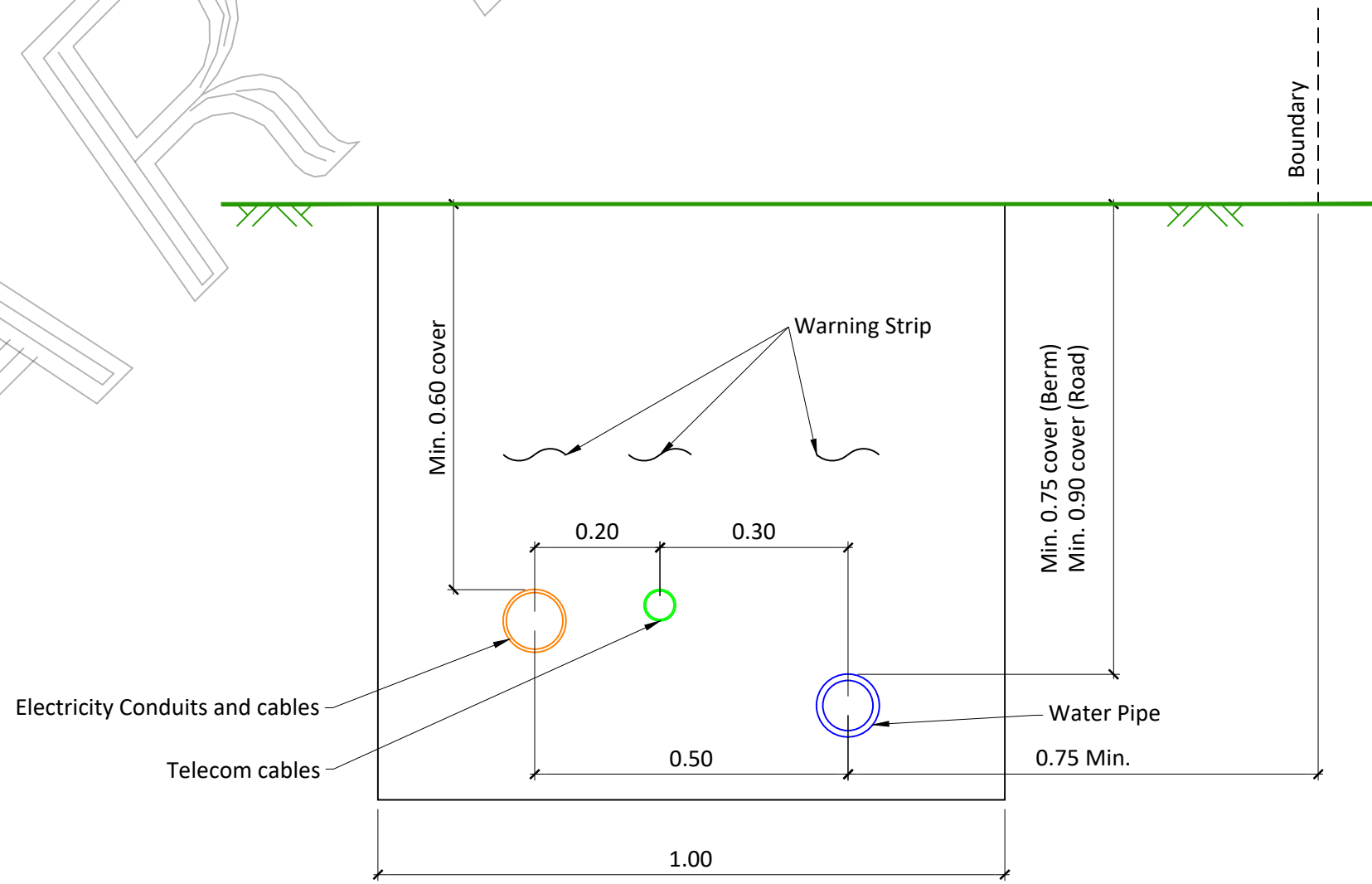
COMMON SERVICES TRENCH DETAIL Scale 1:10
