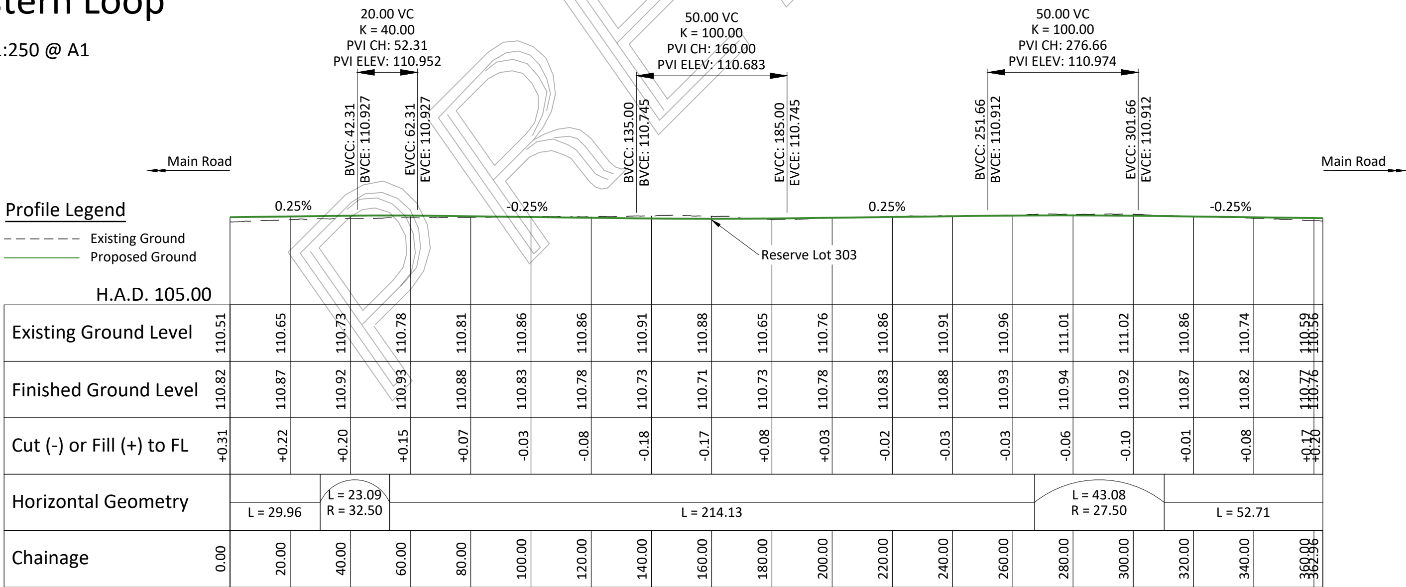
Longsection: Eastern Loop Scale: Horizontal 1:1250; Vertical 1:250 @ A1
